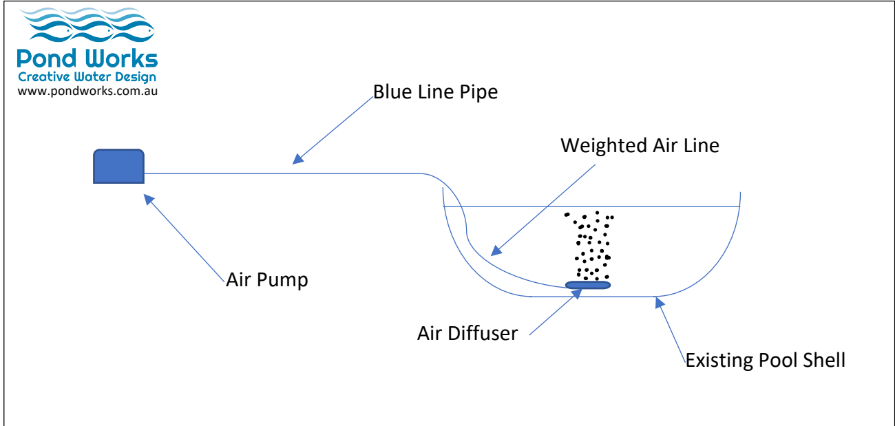
Basic Air Pump set up for Pool to Pond Conversion.
